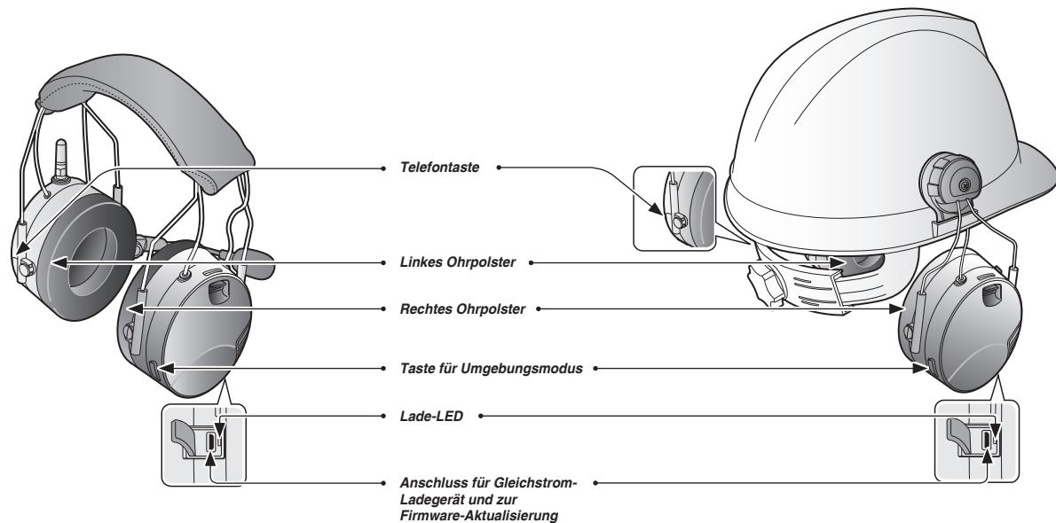
Tufftalk-Headset-Tasten
