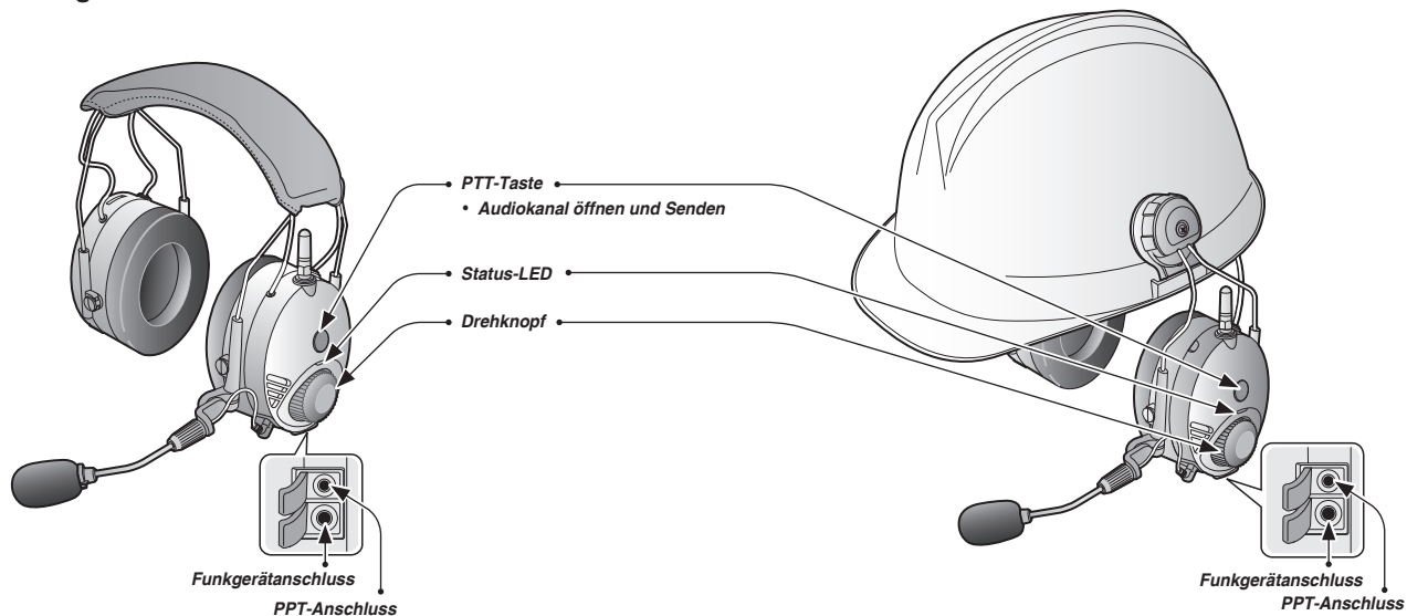
Tufftalk-Headset-Tasten
